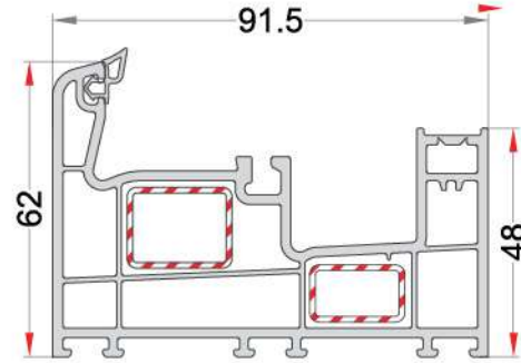
SINGLE RAILED FRAME PROFILE TEK RAYLI KASA PROFİLİ EN 93
