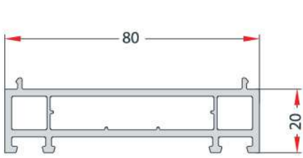
20 x 80 FRAME EXTENSION PROFILE 20 x 80 GENİŞLETME PROFİLİ EN 110 HIGHLINE
