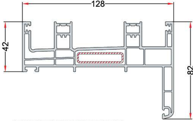
SLIDE WELL SLIDING FRAME PROFILE SLIDE WELL SÜRME KASA PROFİLİ EN 118
