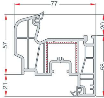
FRAME PROFILE WITH CASING PERVAZLI KASA PROFİLİ EN 20
