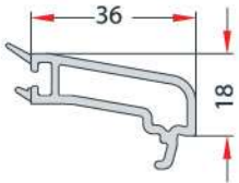
4-mm SINGLE GLAZING BEAD 4 mm TEK CAM ÇİTASI EN 85
