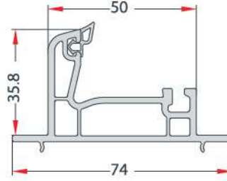
SLIDING FIX PROFILE SABİT PROFİLİ EN 98
