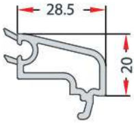
4-mm SINGLE GLAZING BEAD 4 mm TEK CAM ÇİTASI EN 47
