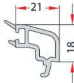
20-mm DOUBLE GLAZING BEAD 20 mm ÇİFT CAM ÇİTASI EN 86
