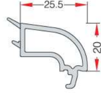
20-mm OVAL DOUBLE GLAZING BEAD 20 mm OVAL ÇİFT CAM ÇİTASI EN 106
