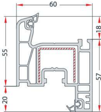
FRAME PROFILE WITH CASING PERVAZLI KASA PROFİLİ EN 87
