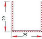
U-TYPE REINFORCEMENT STEEL - U-SAC FRAME - WINDOW SASH - WINDOW SASH WITH DRIP KASA - PENCERE KANAT - DAMLALIKLI KANAT
