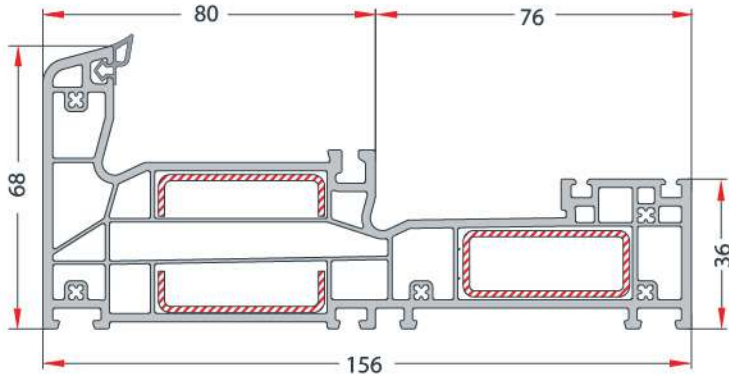
MASTERLINE INSULATED SLIDING FRAME PROFILE MASTERLINE YALITIMLI SÜRME KASA PROFİLİ EN 342
