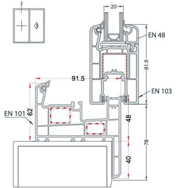
SINGLE RAILED SLIDING FRAME WITH CASING - SLIDING SASH INSTALLATION SÜRME TEK RAYLI PERVAZLI KASA - SÜRME KANAT UYGULAMASI
