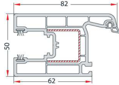
SLIDING SASH PROFILE SÜRME KANAT PROFİLİ EN 95 (without brush seal - kıl fitilsiz) EN 103 (with brush seal - kıl fitilli)
