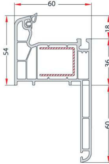
FRAME PROFILE WITH CASING (6 cm) PERVAZLI KASA PROFİLİ (6 cm) EN 873
