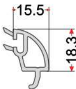
24 mm OVAL DOUBLE GLAZING BEAD 24 mm OVAL ÇİFT CAM ÇİTASI EN 891
