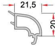
24-mm OVAL DOUBLE GLAZING BEAD 24 mm OVAL ÇİFT CAM ÇİTASI EN 107
