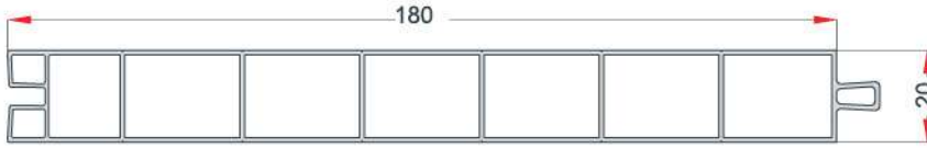
18-cm PANEL PROFILE 18 cm LAMBRI PROFİLİ EN 59
