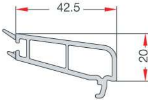
4-mm SINGLE GLAZING BEAD 4 mm TEK CAM ÇİTASI EN 46
