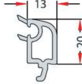
20-mm DOUBLE GLAZING BEAD 20 mm ÇİFT CAM ÇİTASI EN 48
