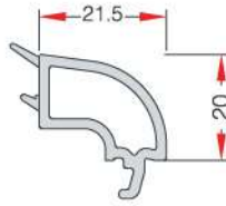
24-mm OVAL DOUBLE GLAZING BEAD 24 mm OVAL ÇİFT CAM ÇİTASI EN 107
