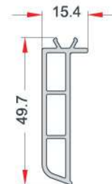
CASING PROFILE WITH CLIP KLİPSLİ PERVAZ PROFİLİ EN 30
