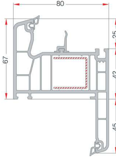
FRAME PROFILE WITH CASING PERVAZLI KASA PROFİLİ EN 711
