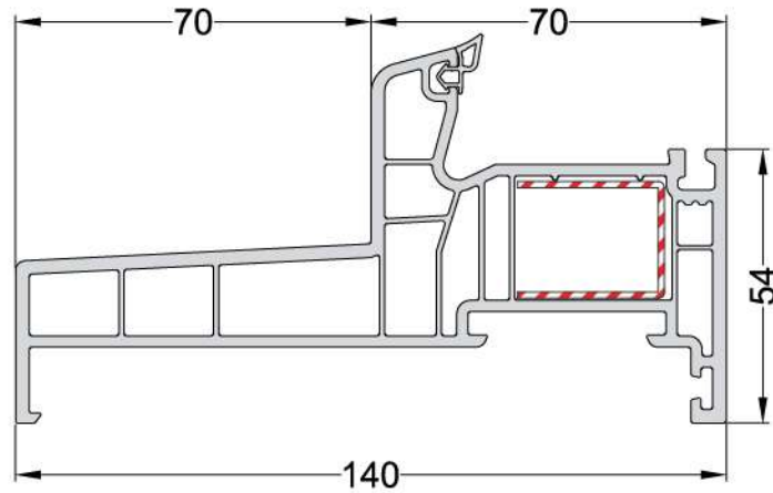
140-mm FRENCH FRAME PROFILE 140 mm FRANSIZ KASA PROFİLİ EN 14
