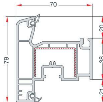
WINDOW SASH WITH DRIP PROFILE DAMLALIKLI PENCERE KANAT PROFİLİ EN 19
