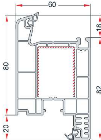
FRAME PROFILE WITH CASING (6 cm) PERVAZLI KASA PROFİLİ (6 cm) EN 873
