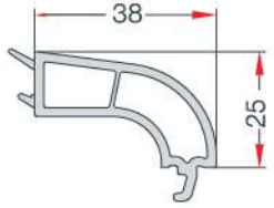
20-mm DOUBLE GLAZING BEAD 20 mm ÇİFT CAM ÇİTASI EN 76
