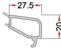
20-mm DOUBLE GLAZING BEAD 20 mm ÇİFT CAM ÇİTASI EN 45
