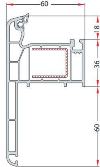
ASYMETRIC FRAME PROFILE WITH CASING (6 cm) ASİMETRİK PERVAZLI KASA PROFİLİ (6 cm) EN 874
