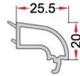
20-mm OVAL DOUBLE GLAZING BEAD 20 mm OVAL ÇİFT CAM ÇİTASI EN 106
