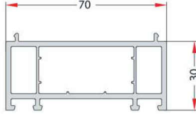
30 x 70 FRAME EXTENSION PROFILE 30 x 70 GENİŞLETME PROFİLİ EN 111 KLASLINE
