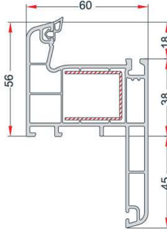
FRAME PROFILE WITH CASING PERVAZLI KASA PROFİLİ EN 872
