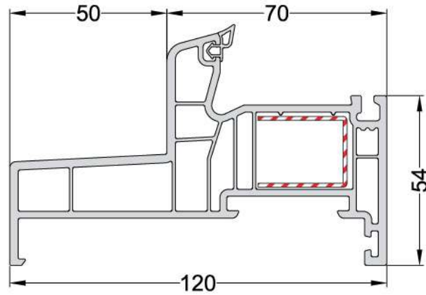
120-mm FRENCH FRAME PROFILE 120 mm FRANSIZ KASA PROFİLİ EN 13
