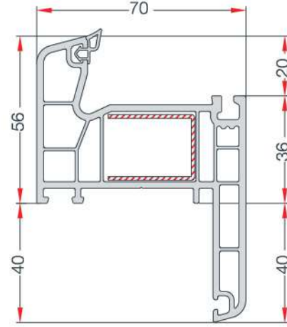
FRAME PROFILE WITH CASING PERVAZLI KASA PROFİLİ EN 108
