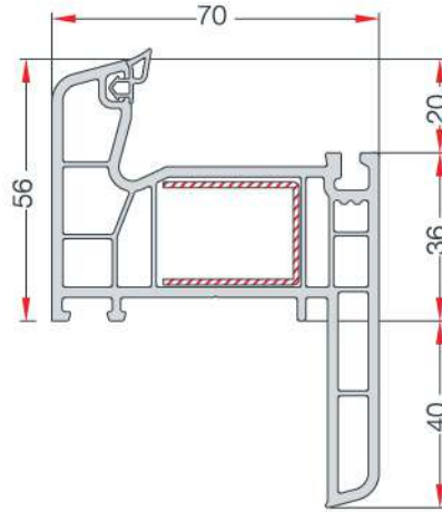
FRAME PROFILE WITH CASING PERVAZLI KASA PROFİLİ EN 20
