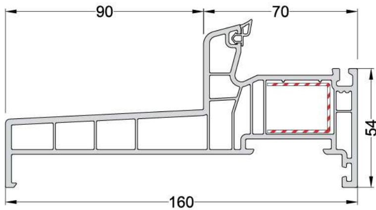
160-mm FRENCH FRAME PROFILE 160 mm FRANSIZ KASA PROFİLİ EN 15
