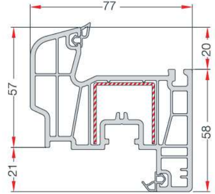
WINDOW SASH WITH DRIP PROFILE DAMLALIKLI PENCERE KANAT PROFİLİ EN 19
