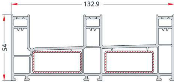
TRIPLE RAILED SLIDING FRAME PROFILE ÜÇ RAYLI KASA PROFİLİ EN 104
