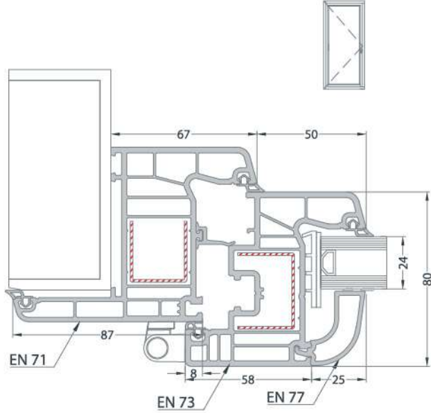
FRAME WITH CASING - WINDOW SASH INSTALLATION PERVAZLI KASA - PENCERE KANAT UYGULAMASI
