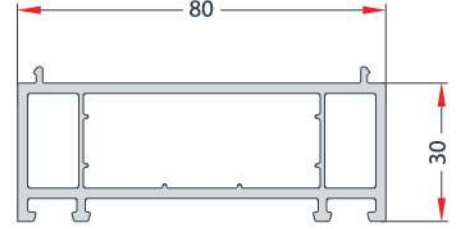
30 x 80 FRAME EXTENSION PROFILE 30 x 80 GENİŞLETME PROFİLİ EN 112 HIGHLINE
