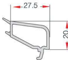
20-mm DOUBLE GLAZING BEAD 20 mm ÇİFT CAM ÇİTASI EN 45
