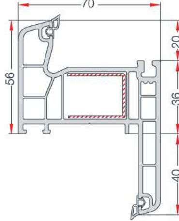
FRAME PROFILE WITH CASING PERVAZLI KASA PROFİLİ EN 203
